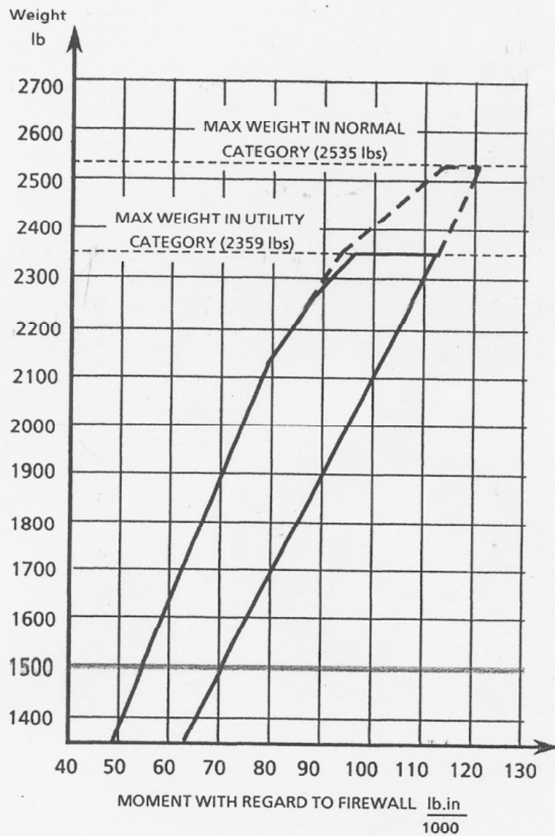
Figure 6.5 - LIMITS WEIGHT / MOMENT
